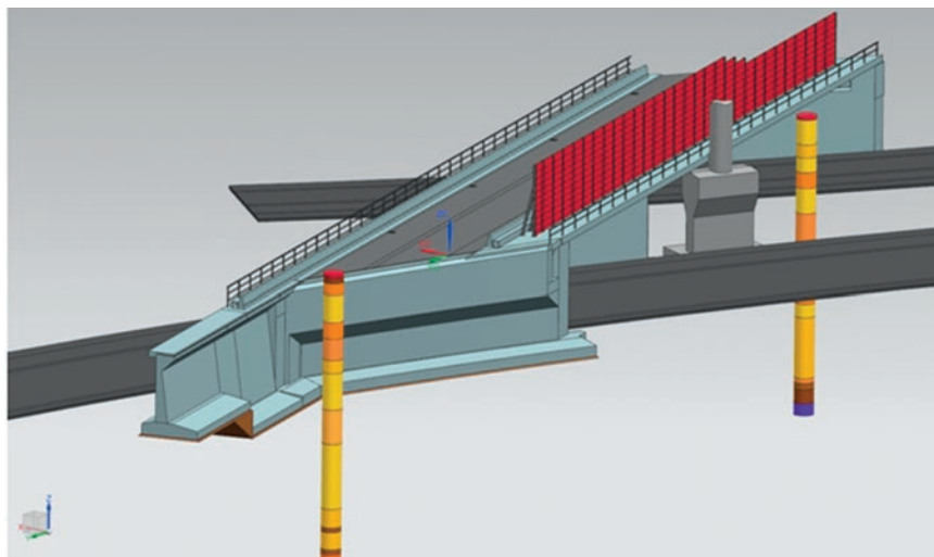
Geometry model “duraBASt” bridge
